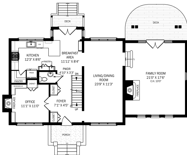
CEILING HEIGHT 8'3" MAIN FLOOR - 1289 SQUARE FEET
